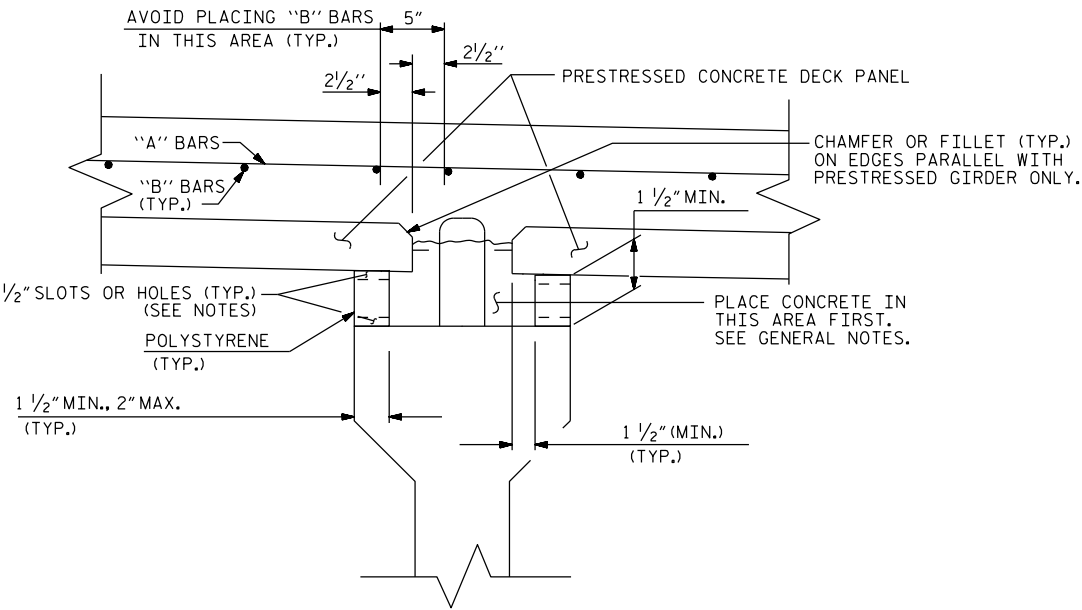
POLYSTYRENE SUPPORT
